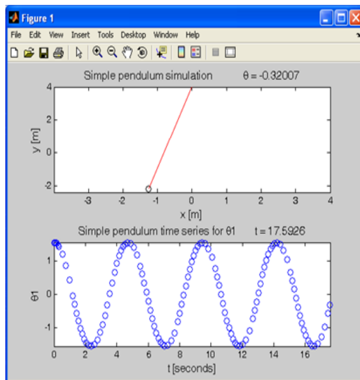
Figure 4: Simple pendulum and its time series
