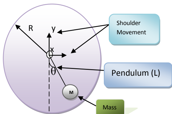
Fig.3: Movement of pendulum as energy generator
