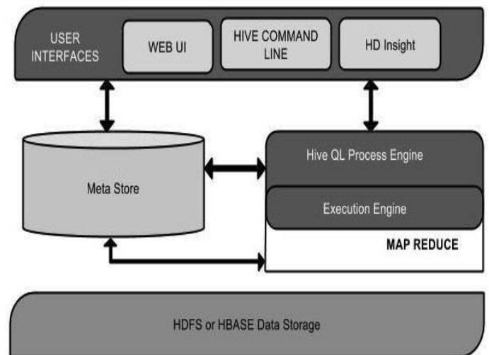
Figure 1. Hive architecture
